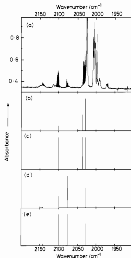
Figure 3. Comparison of (a) the IR spectrum observed for A in the \nu(\text{C}-\text{O}) region (Ar:O 2 :Fe(CO) 5 = ca. 2000:100:1; photolysis for 40 min at \lambda = ca. 312 nm; bands due to A distinguished by black infilling) with schematic representations of the corresponding spectra characteristic of the following units: (b) \text{Fe}(\text{CO})_3 with C_{2v} symmetry (model XII); (c) \text{Fe}(\text{CO})_3 with C_{3v} symmetry (model XIII); (d) \text{Fe}(\text{CO})_4 with C_{2v} symmetry (model XIV); and (e) \text{Fe}(\text{CO})_4 with C_{3v} symmetry (model XV).
