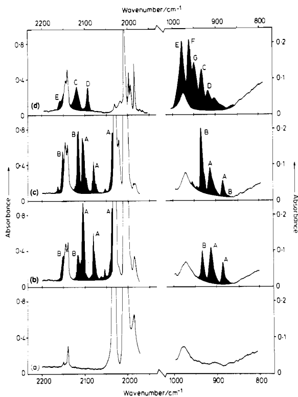
Figure 1. IR spectrum of \text{Fe}(\text{CO})_5 isolated in an \text{O}_2 -doped Ar matrix ( \text{Ar}:\text{O}_2:\text{Fe}(\text{CO})_5 = \text{ca. } 1000:50:1 ) in the regions 1950\text{--}2200 and 800\text{--}1000\text{ cm}^{-1} showing the effects of photolysis at wavelengths near 312\text{ nm} : (a) after deposition, (b) after 60 min of photolysis, (c) after 160 min of photolysis, and (d) after 360 min of photolysis at \lambda = \text{ca. } 312\text{ nm} followed by a further 200 min of photolysis using a \text{Br}_2 filter ( 290 \leq \lambda \leq 370 and \lambda \geq 550\text{ nm} ). Bands with black infilling are due to the products A–G. The broad band centered near 970\text{ cm}^{-1} in these and other spectra is associated with an impurity on or in the CsI window.
